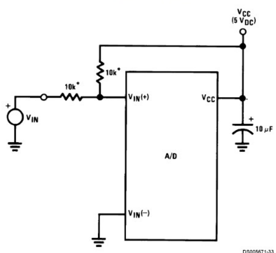
Handling \pm 5V Analog Inputs
