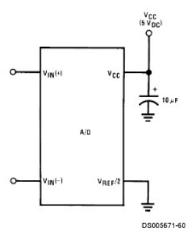
A \mu P Interfaced Comparator
