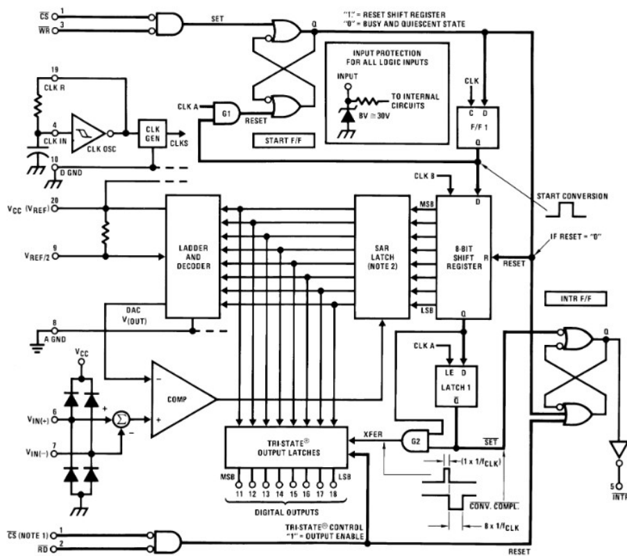
FIGURE 4. Block Diagram
