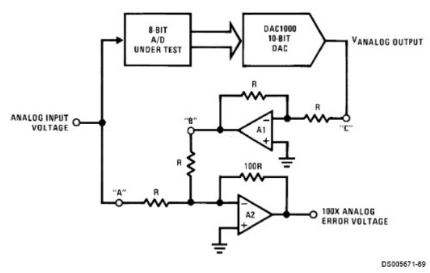
FIGURE 10. A/D Tester with Analog Error Output
