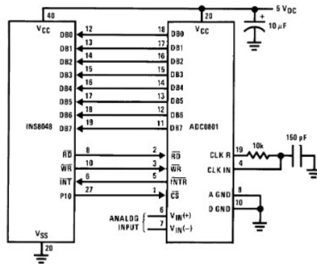
FIGURE 13. INS8048 Interface
