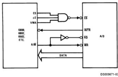
6800 Interface
