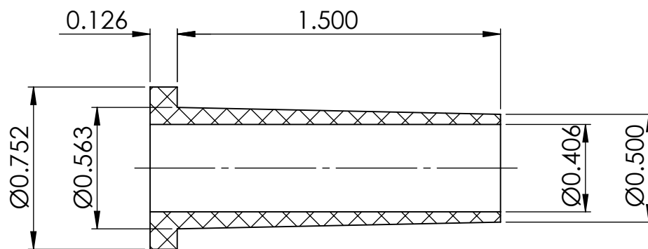
SECTION Y-Y
