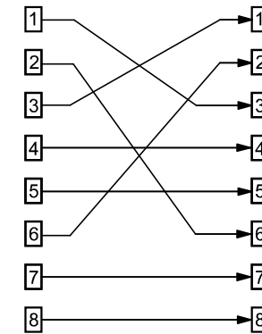
10/100BASE-T (TIA568B)
