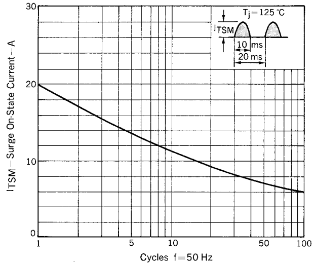
Fig. 10 I_{TSM} RATINGS
